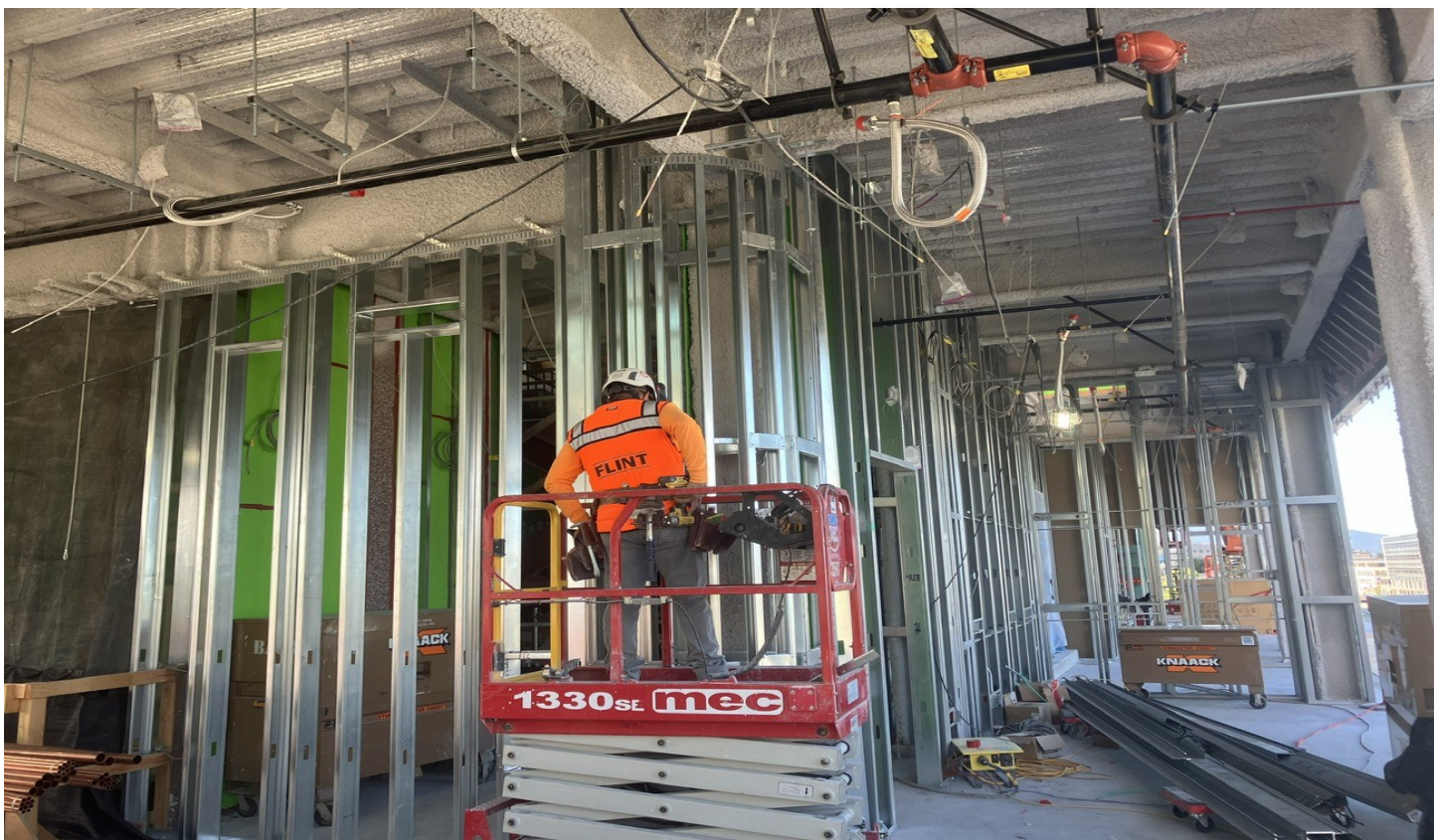
Level 4 Interior Framing
